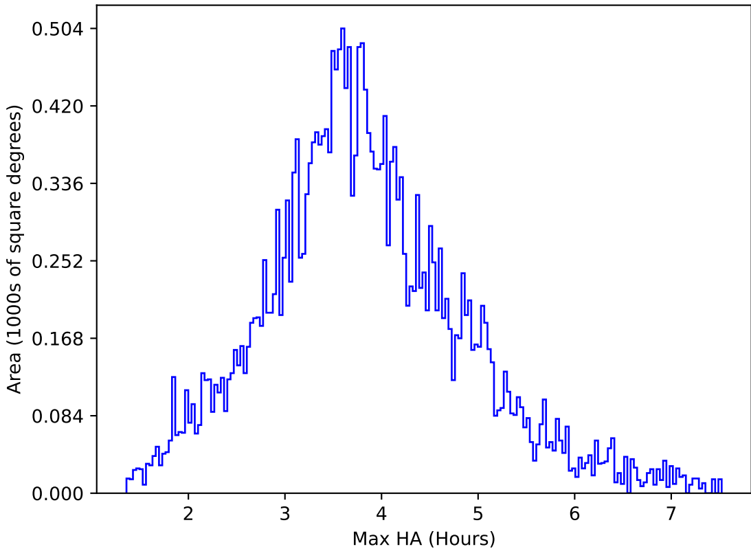
ddf_acor_sf15_lsf30_lsr10_v3.4_10yrs All sky g band: Max HA
