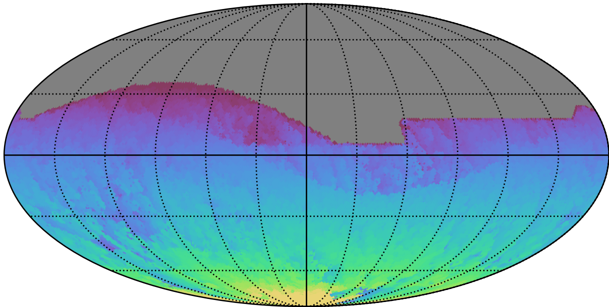
ddf_acor_sf15_lsf30_lsr10_v3.4_10yrs All sky all bands: Max HA
