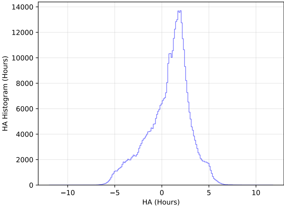
ddf_acor_sf15_lsf30_lsr10_v3.4_10yrs WFD z band: HA Histogram
