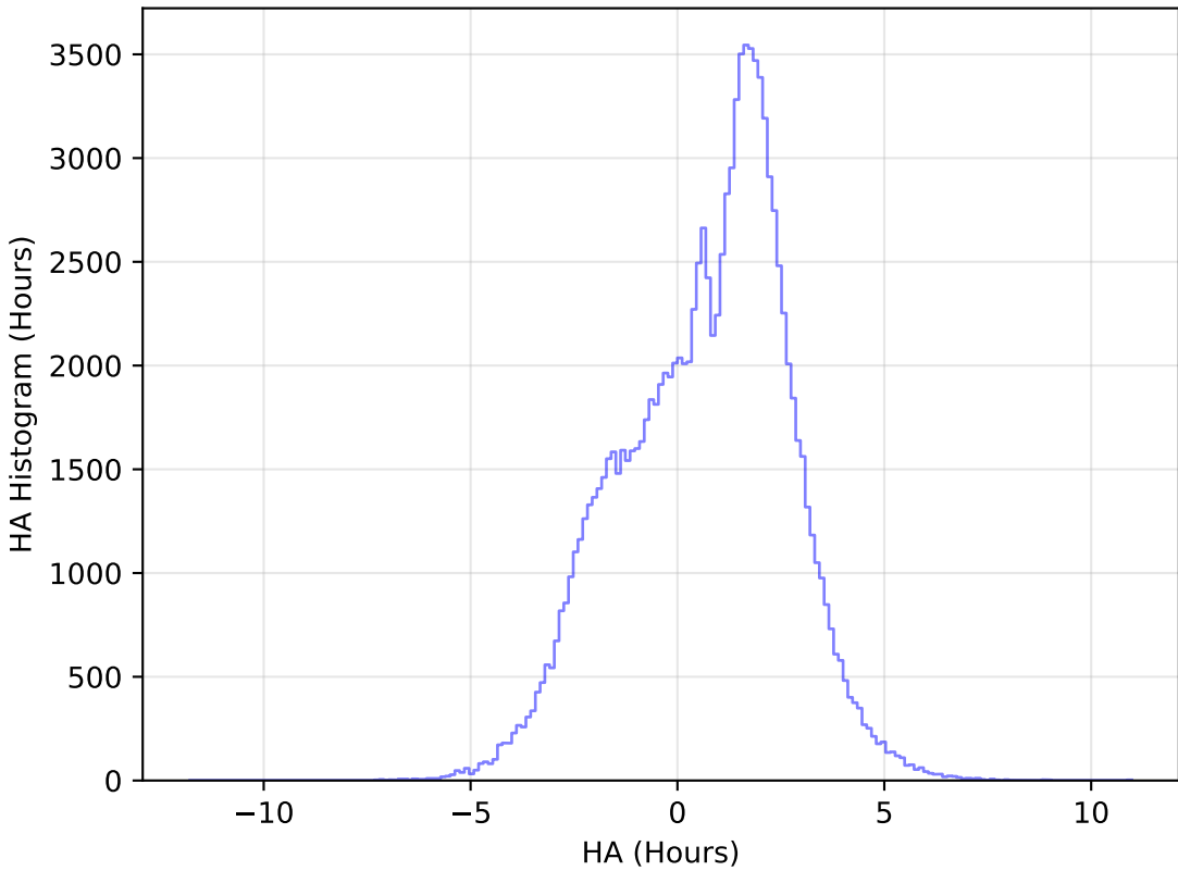
ddf_acor_sf15_lsf30_lsr10_v3.4_10yrs WFD u band: HA Histogram
