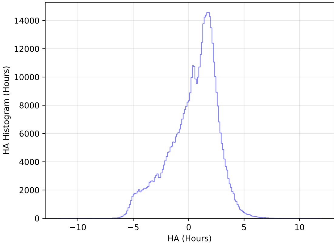
ddf_acor_sf15_lsf30_lsr10_v3.4_10yrs WFD r band: HA Histogram
