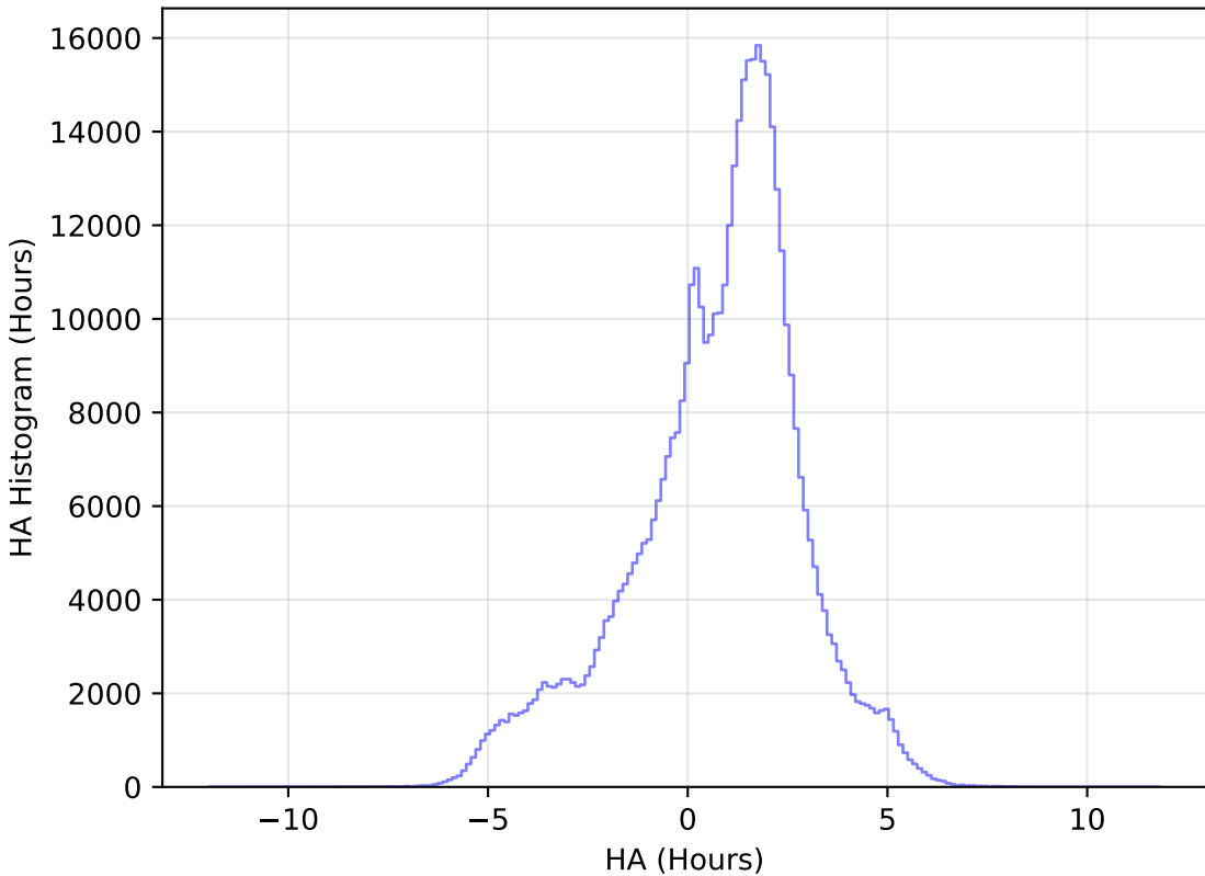
ddf_acor_sf15_lsf30_lsr10_v3.4_10yrs WFD i band: HA Histogram
