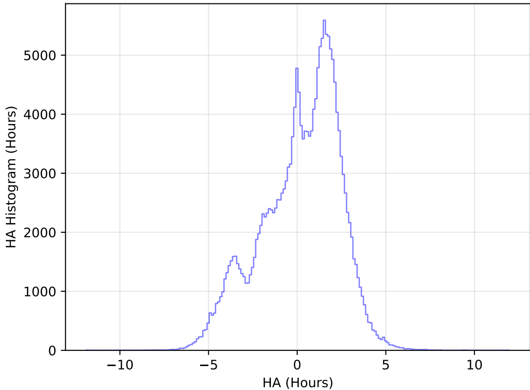
ddf_acor_sf15_lsf30_lsr10_v3.4_10yrs WFD g band: HA Histogram
