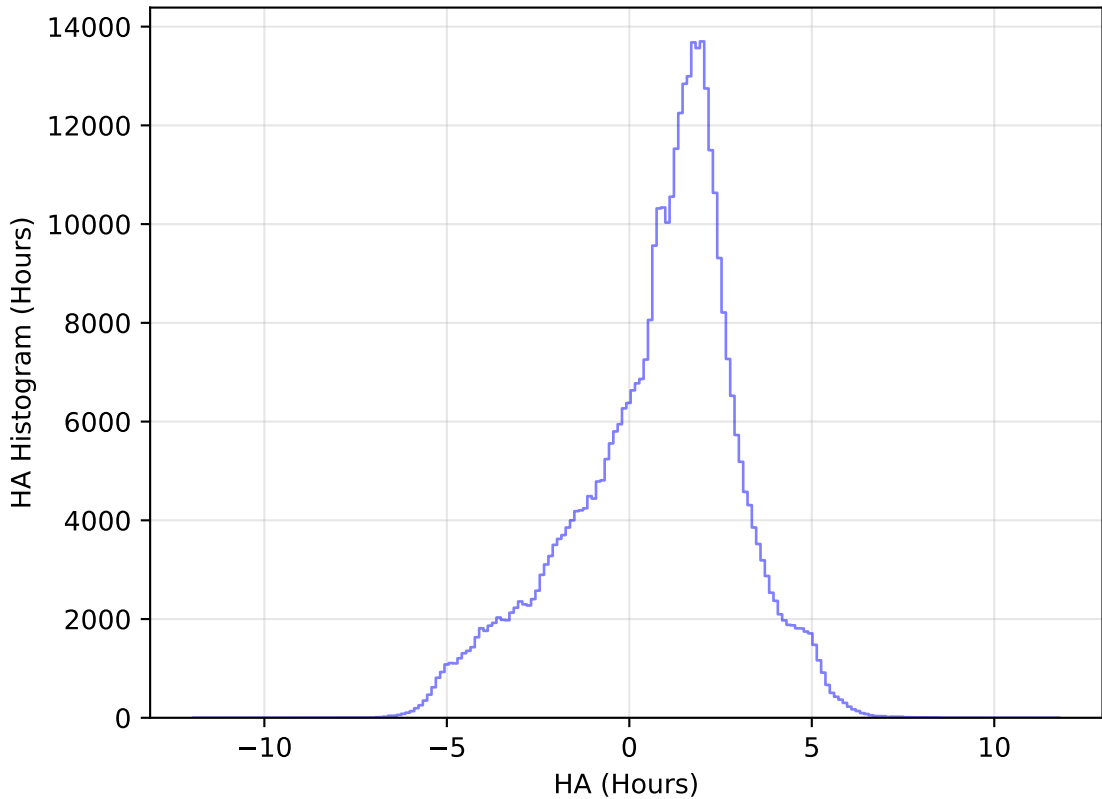
ddf_acor_sf15_lsf30_lsr10_v3.4_10yrs All sky z band: HA Histogram
