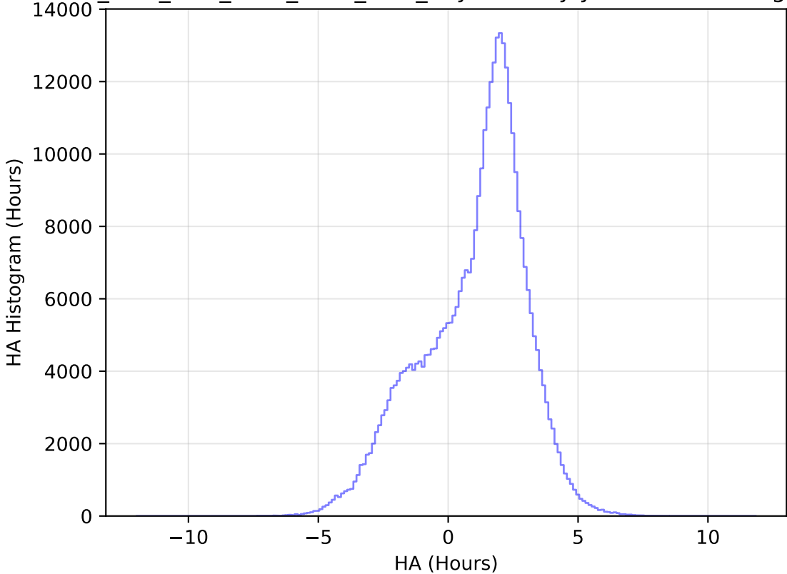
ddf_acor_sf15_lsf30_lsr10_v3.4_10yrs All sky y band: HA Histogram
