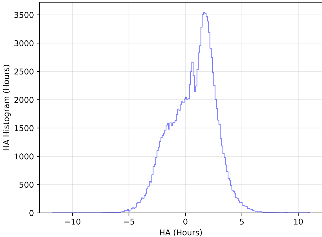
ddf_acor_sf15_lsf30_lsr10_v3.4_10yrs All sky u band: HA Histogram
