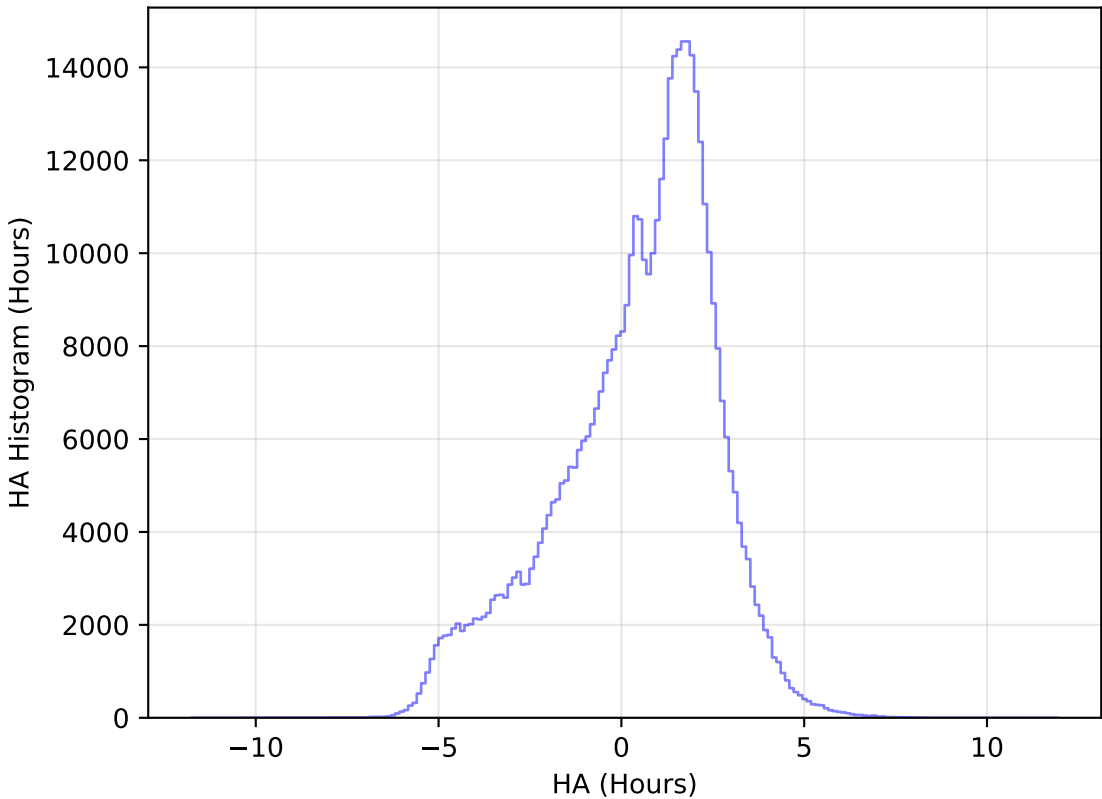
ddf_acor_sf15_lsf30_lsr10_v3.4_10yrs All sky r band: HA Histogram
