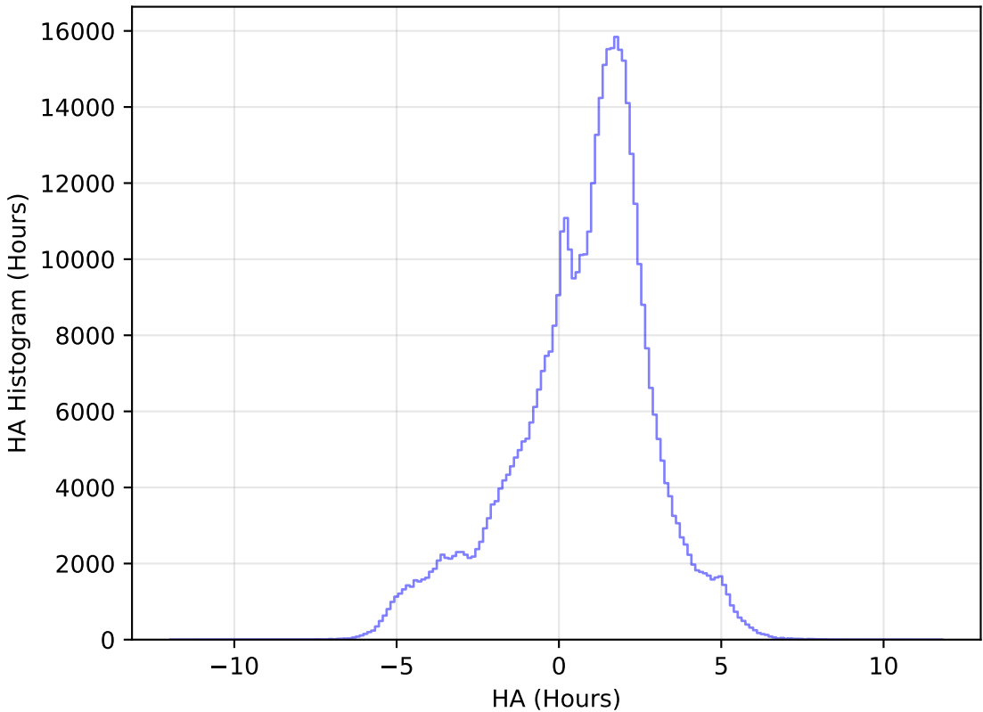
ddf_acor_sf15_lsf30_lsr10_v3.4_10yrs All sky i band: HA Histogram
