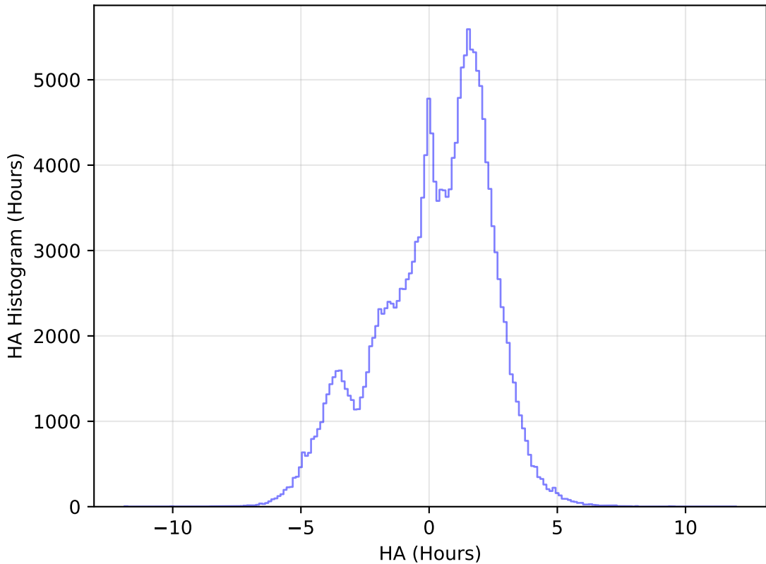
ddf_acor_sf15_lsf30_lsr10_v3.4_10yrs All sky g band: HA Histogram
