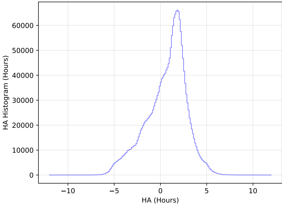
ddf_acor_sf15_lsf30_lsr10_v3.4_10yrs All sky all bands: HA Histogram
