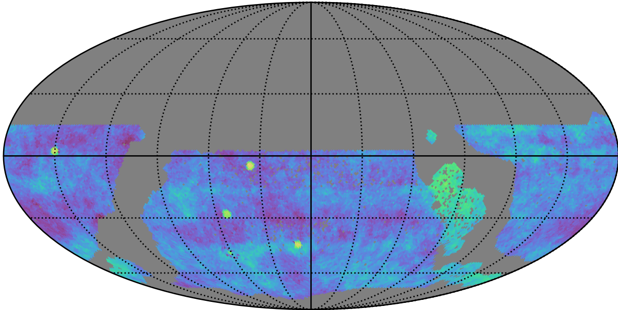
ddf_acor_sf15_lsf30_lsr10_v3.4_10yrs gri WFD: Fraction of visits in pairs (20-90 min)
