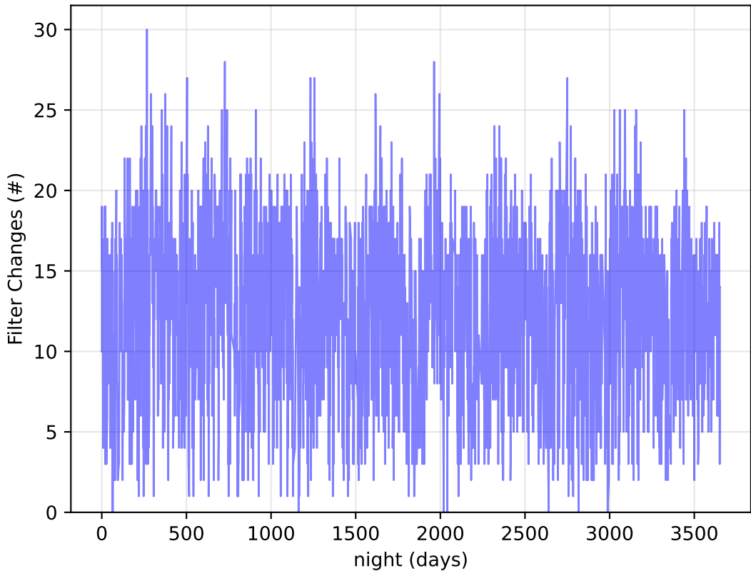
ddf_acor_sf15_lsf30_lsr10_v3.4_10yrs Per Night: Filter Changes
