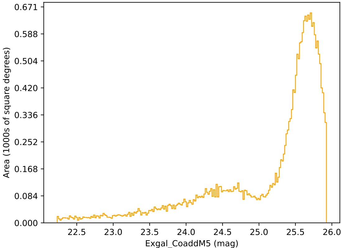
ddf_acor_sf15_lsf30_lsr10_v3.4_10yrs Yr 1 r band: Exgal_CoaddM5
