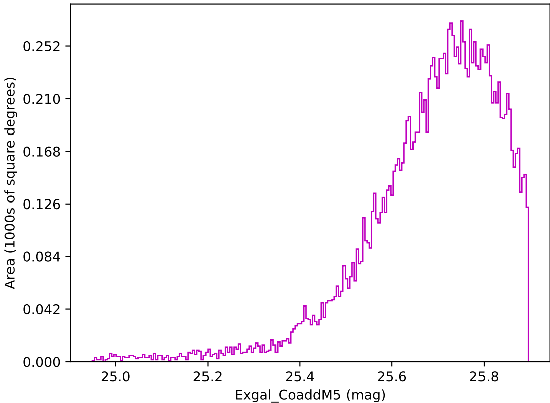
ddf_acor_sf15_lsf30_lsr10_v3.4_10yrs WFD z band: Exgal_CoaddM5
