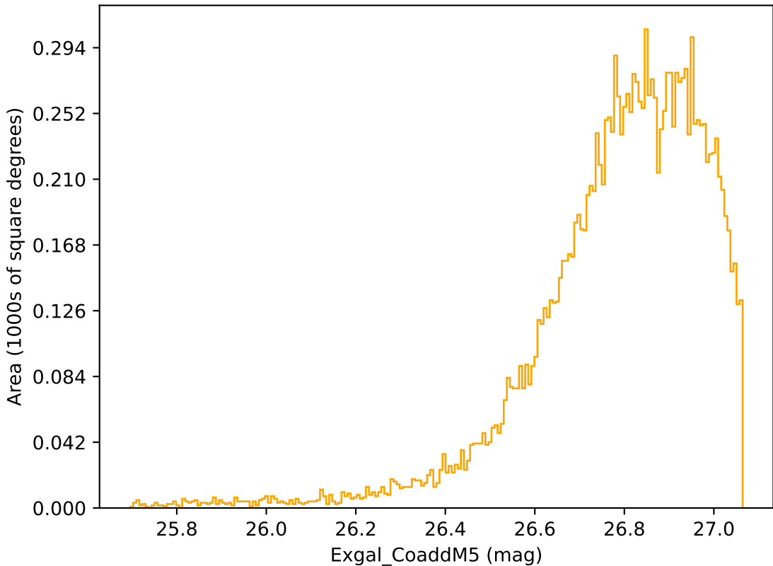
ddf_acor_sf15_lsf30_lsr10_v3.4_10yrs WFD r band: Exgal_CoaddM5
