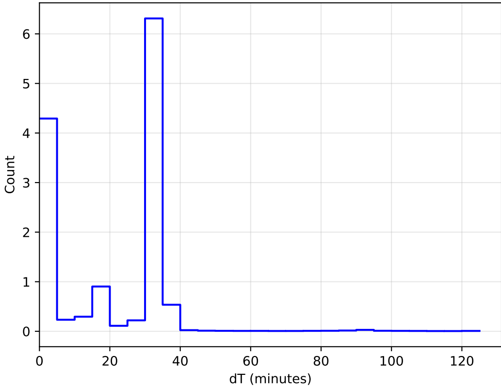
ddf_acor_sf15_lsf30_lsr10_v3.4_10yrs All sky: DeltaT Histogram
