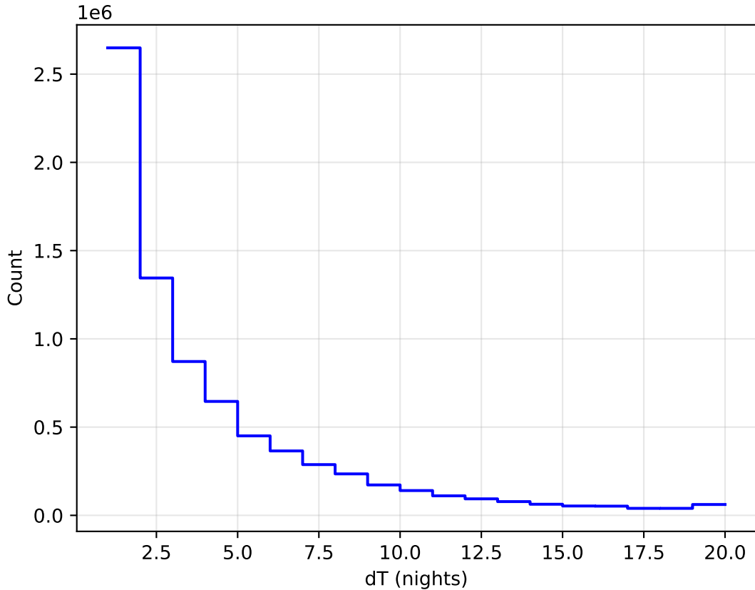
ddf_acor_sf15_lsf30_lsr10_v3.4_10yrs WFD all bands: DeltaNight Histogram
