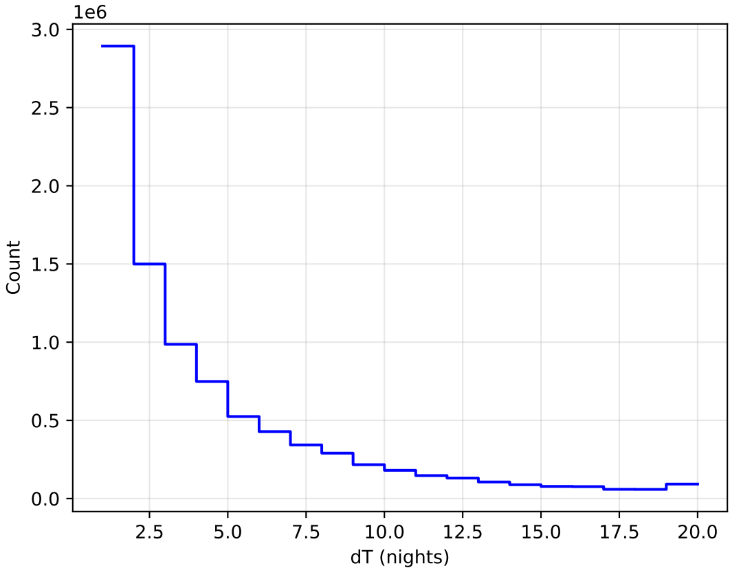
ddf_acor_sf15_lsf30_lsr10_v3.4_10yrs All sky all bands: DeltaNight Histogram
