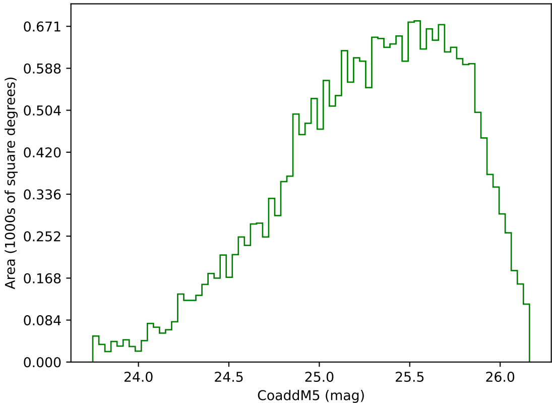
ddf_acor_sf15_lsf30_lsr10_v3.4_10yrs Yr 3-4 g band: CoaddM5
