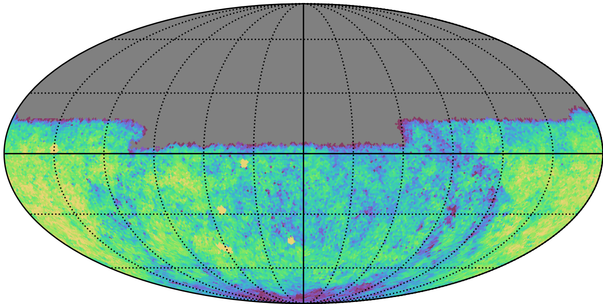
ddf_acor_sf15_lsf30_lsr10_v3.4_10yrs Yr 1 u band: CoaddM5
