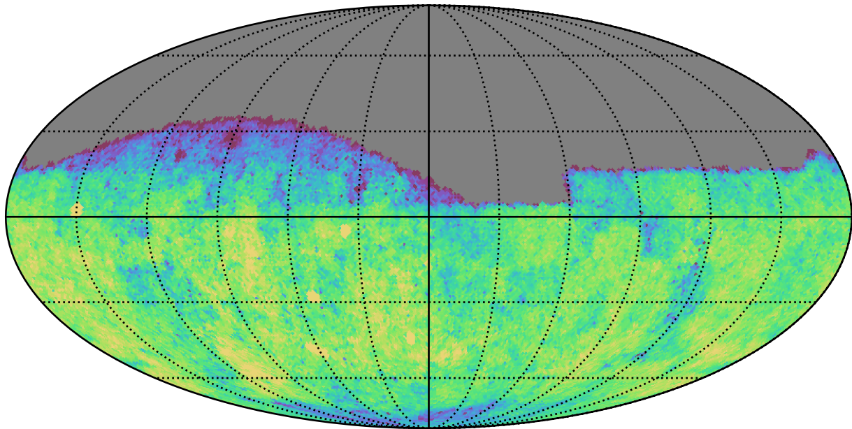
ddf_acor_sf15_lsf30_lsr10_v3.4_10yrs Yr 1 g band: CoaddM5
