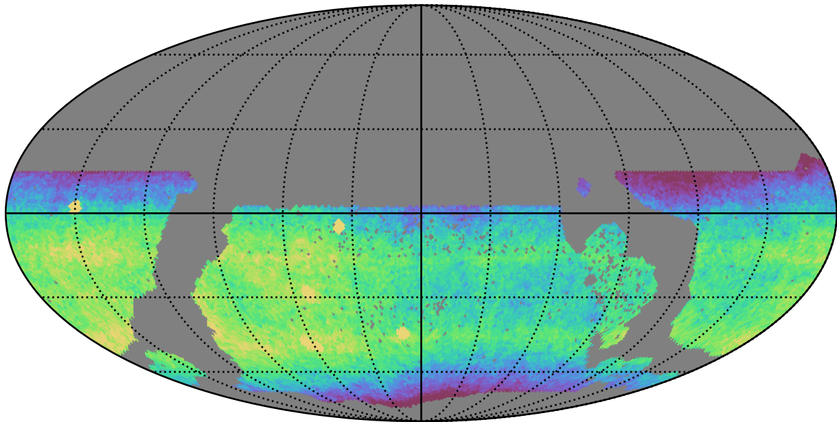
ddf_acor_sf15_lsf30_lsr10_v3.4_10yrs WFD i band: CoaddM5
