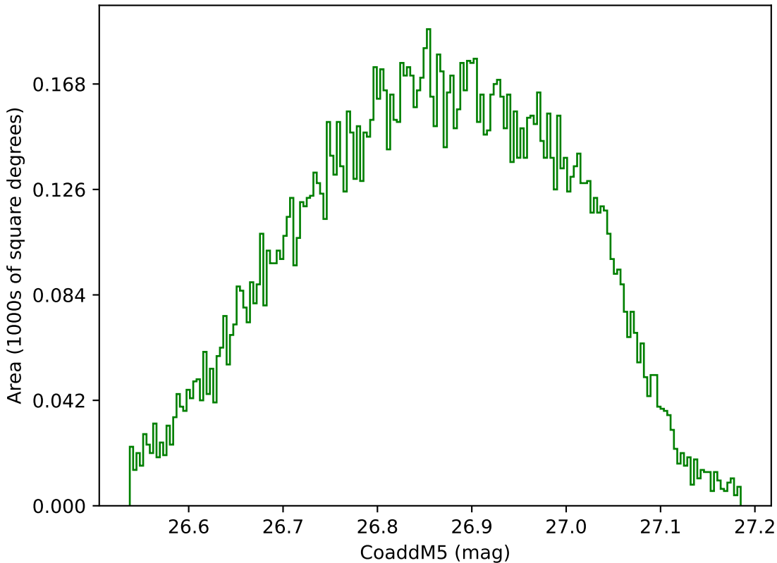
ddf_acor_sf15_lsf30_lsr10_v3.4_10yrs WFD g band: CoaddM5
