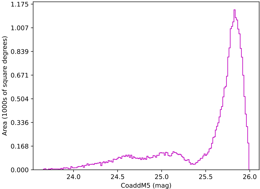
ddf_acor_sf15_lsf30_lsr10_v3.4_10yrs All sky z band: CoaddM5
