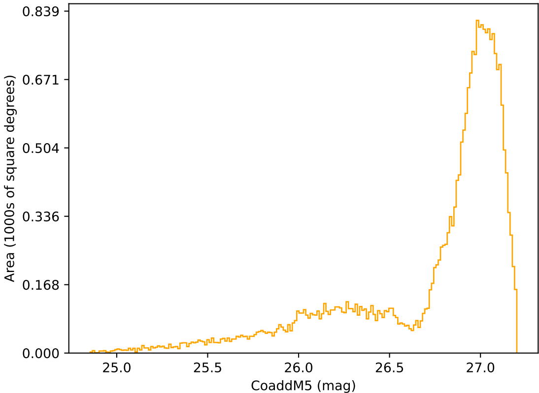
ddf_acor_sf15_lsf30_lsr10_v3.4_10yrs All sky r band: CoaddM5
