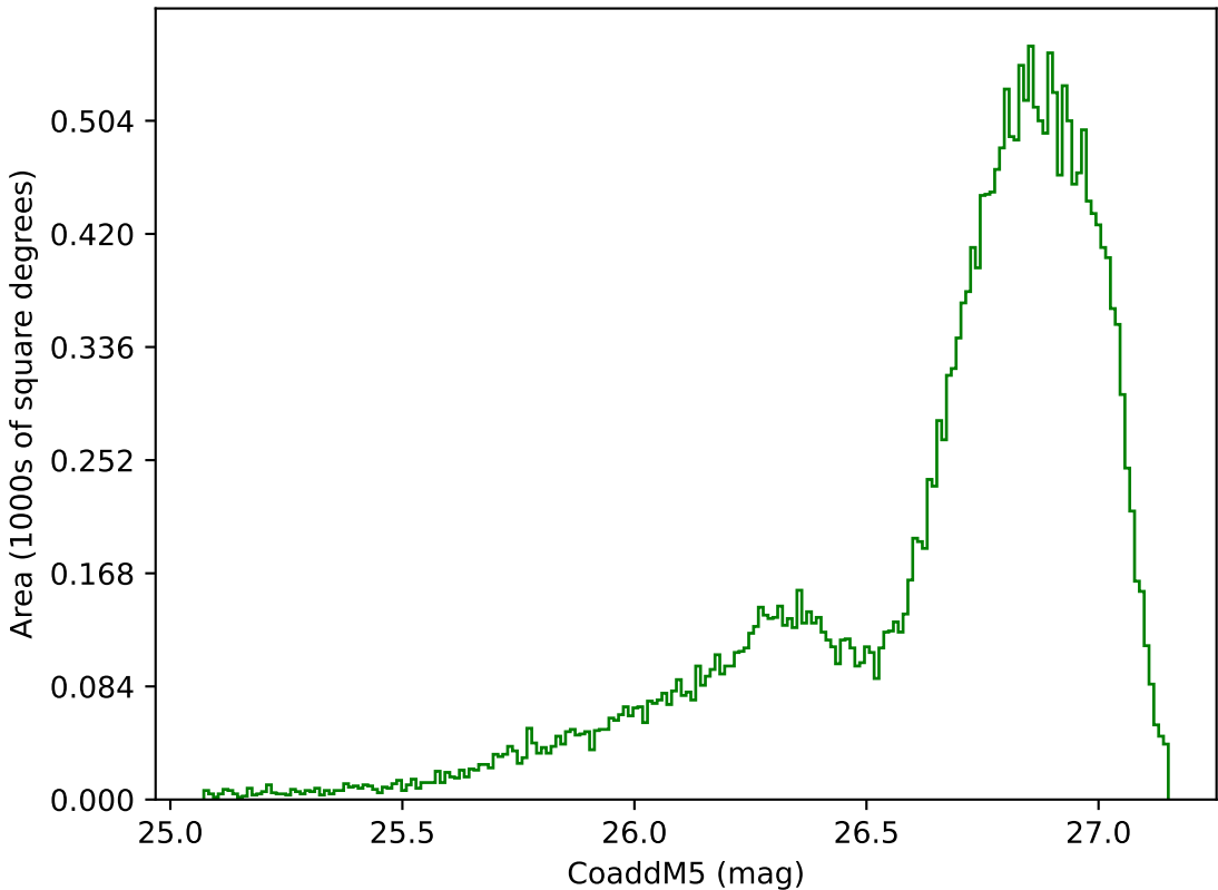
ddf_acor_sf15_lsf30_lsr10_v3.4_10yrs All sky g band: CoaddM5
