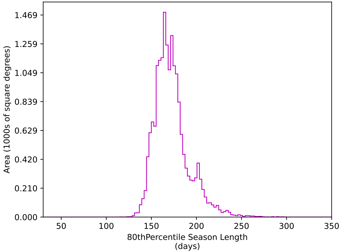
ddf_acor_sf15_lsf30_lsr10_v3.4_10yrs WFD z band: 80thPercentile Season Length
