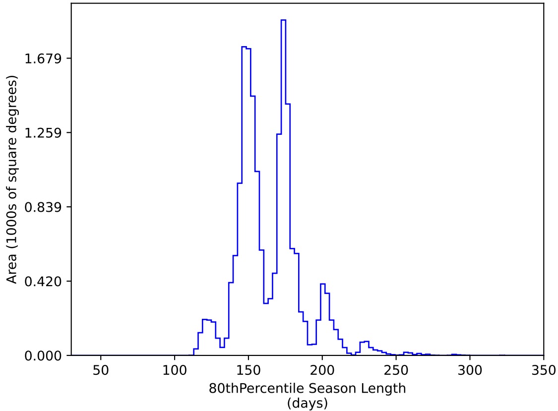
ddf_acor_sf15_lsf30_lsr10_v3.4_10yrs WFD y band: 80thPercentile Season Length
