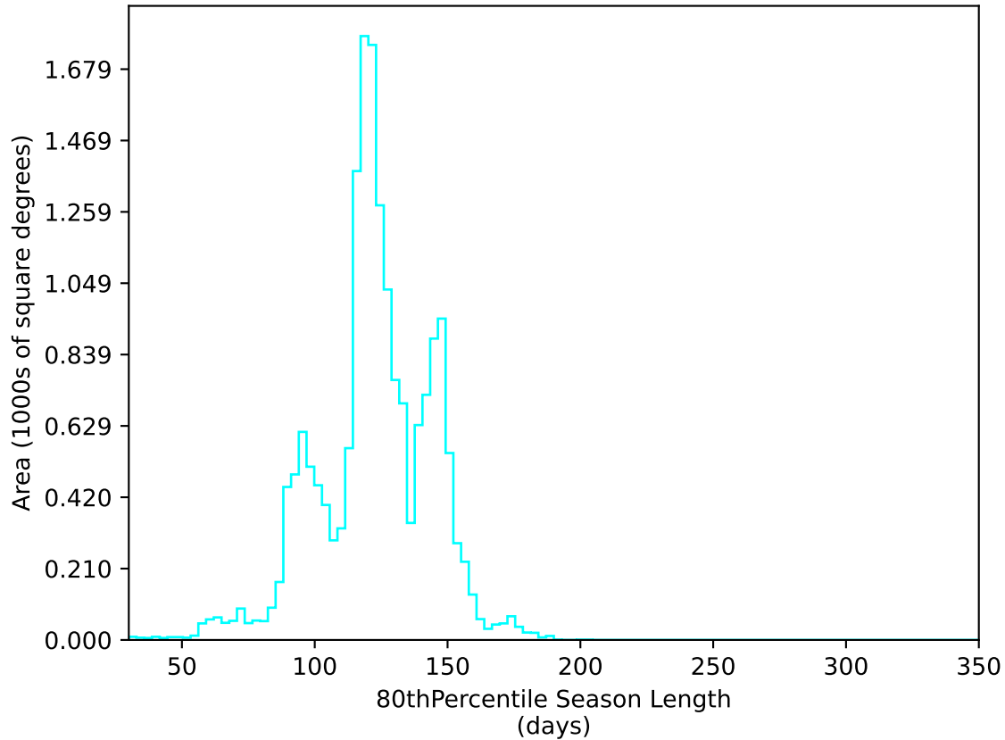
ddf_acor_sf15_lsf30_lsr10_v3.4_10yrs WFD u band: 80thPercentile Season Length
