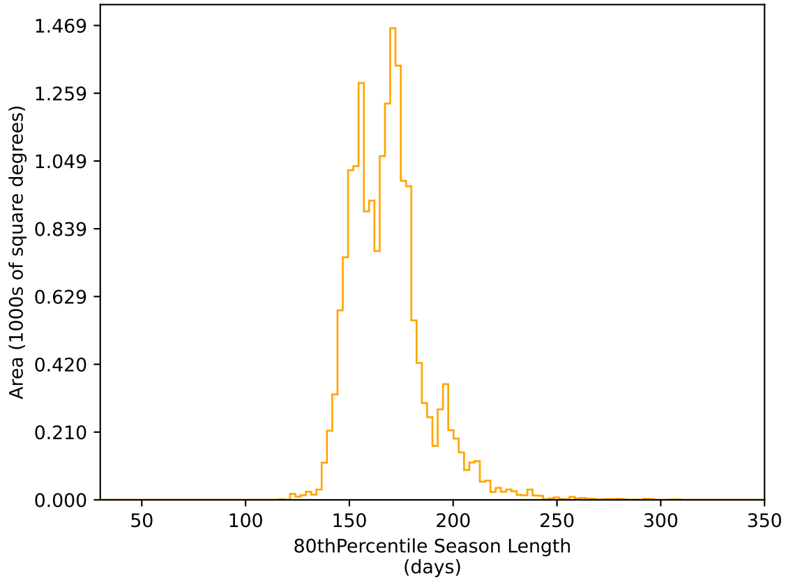
ddf_acor_sf15_lsf30_lsr10_v3.4_10yrs WFD r band: 80thPercentile Season Length
