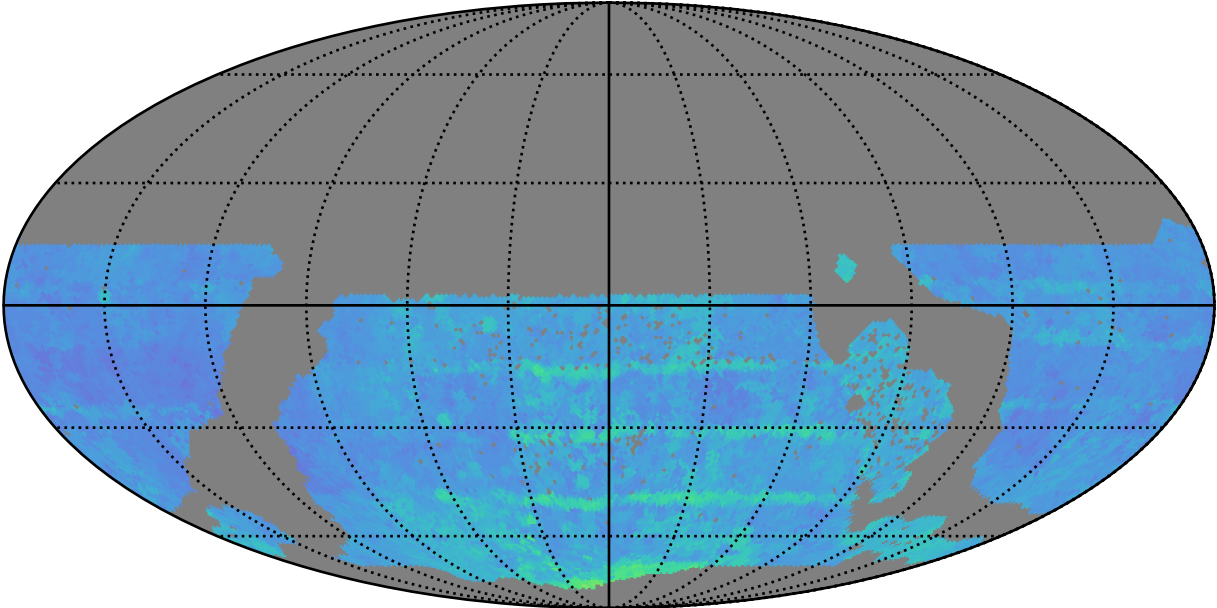
ddf_acor_sf15_lsf30_lsr10_v3.4_10yrs WFD i band: 80thPercentile Season Length
