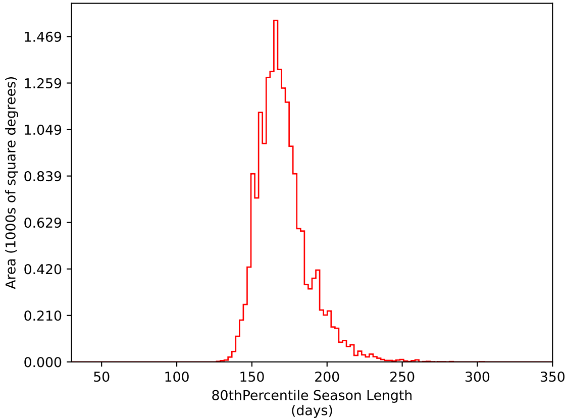
ddf_acor_sf15_lsf30_lsr10_v3.4_10yrs WFD i band: 80thPercentile Season Length
