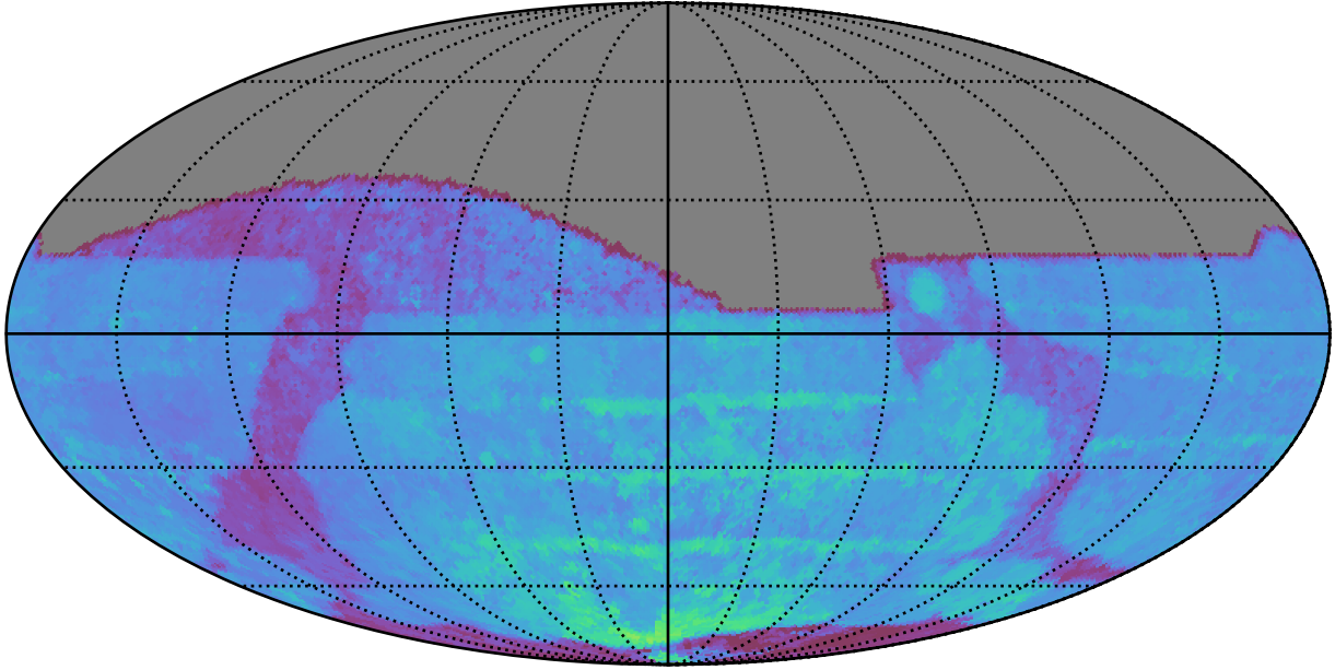
ddf_acor_sf15_lsf30_lsr10_v3.4_10yrs All sky z band: 80thPercentile Season Length
