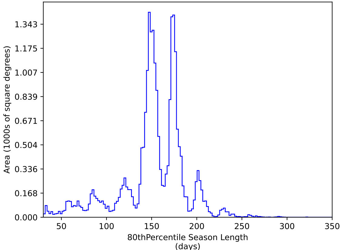
ddf_acor_sf15_lsf30_lsr10_v3.4_10yrs All sky y band: 80thPercentile Season Length
