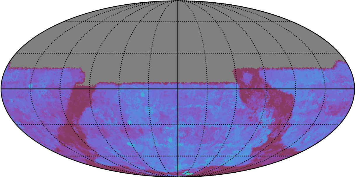
ddf_acor_sf15_lsf30_lsr10_v3.4_10yrs All sky u band: 80thPercentile Season Length
