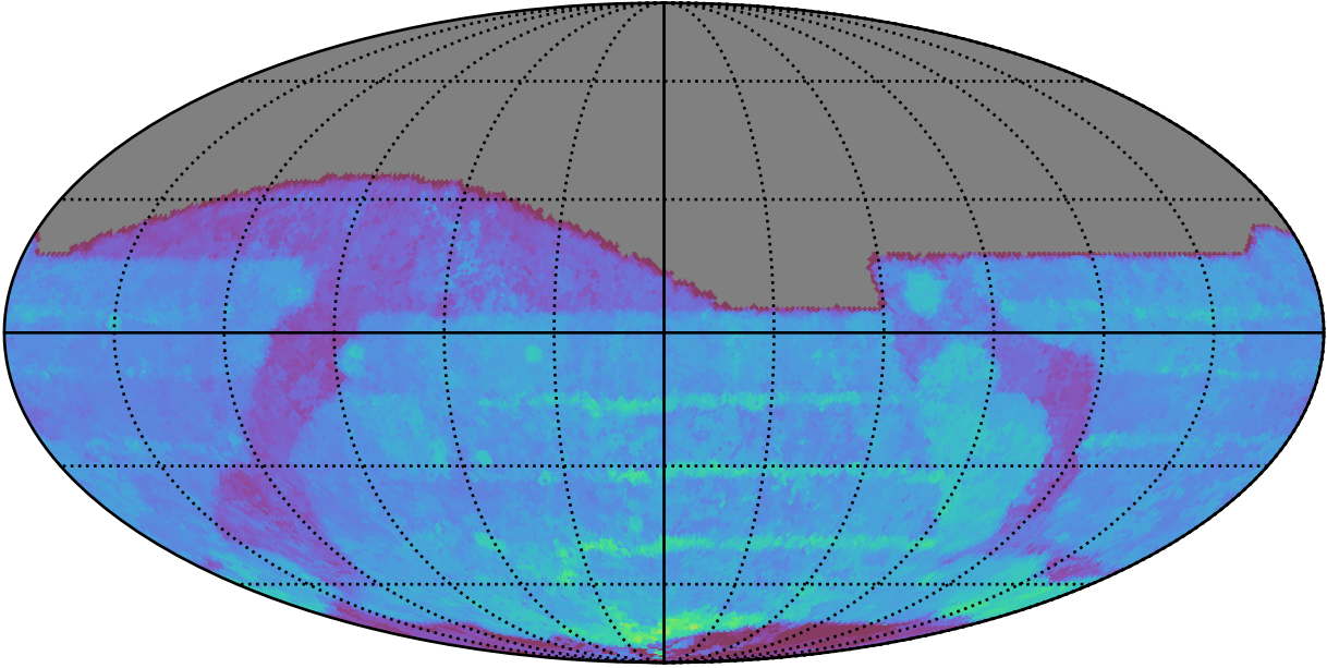
ddf_acor_sf15_lsf30_lsr10_v3.4_10yrs All sky r band: 80thPercentile Season Length
