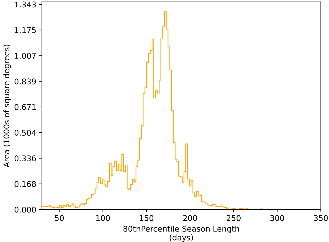
ddf_acor_sf15_lsf30_lsr10_v3.4_10yrs All sky r band: 80thPercentile Season Length
