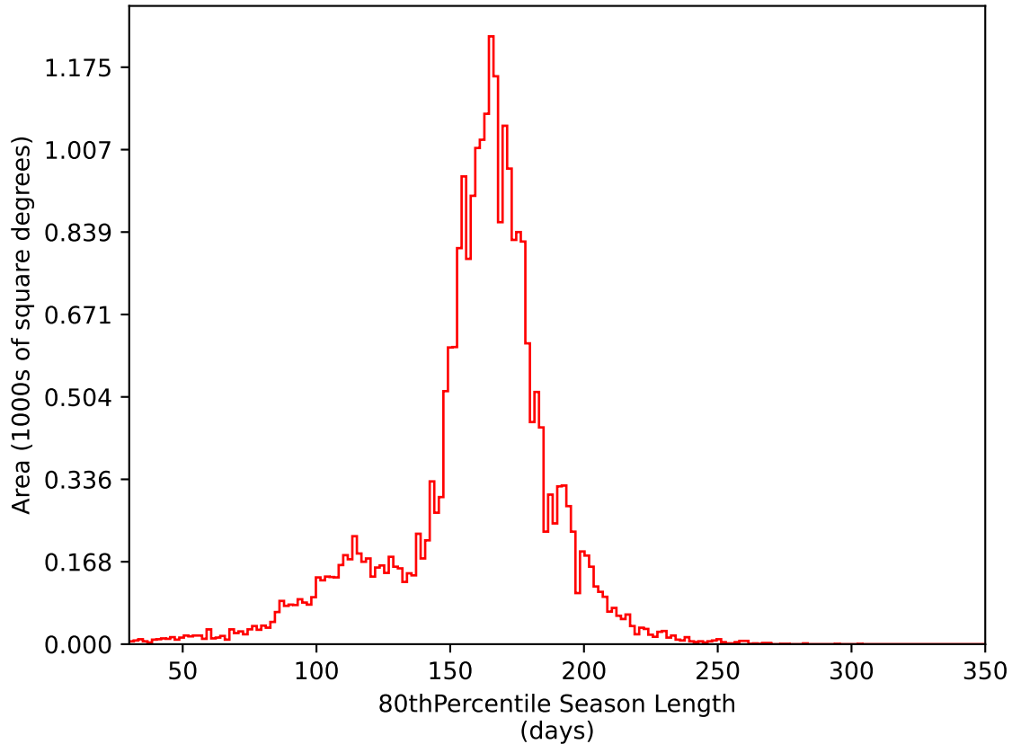
ddf_acor_sf15_lsf30_lsr10_v3.4_10yrs All sky i band: 80thPercentile Season Length
