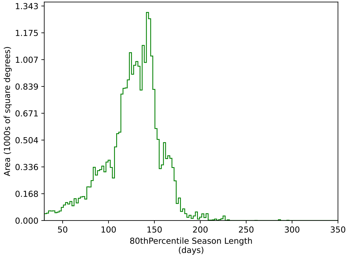
ddf_acor_sf15_lsf30_lsr10_v3.4_10yrs All sky g band: 80thPercentile Season Length
