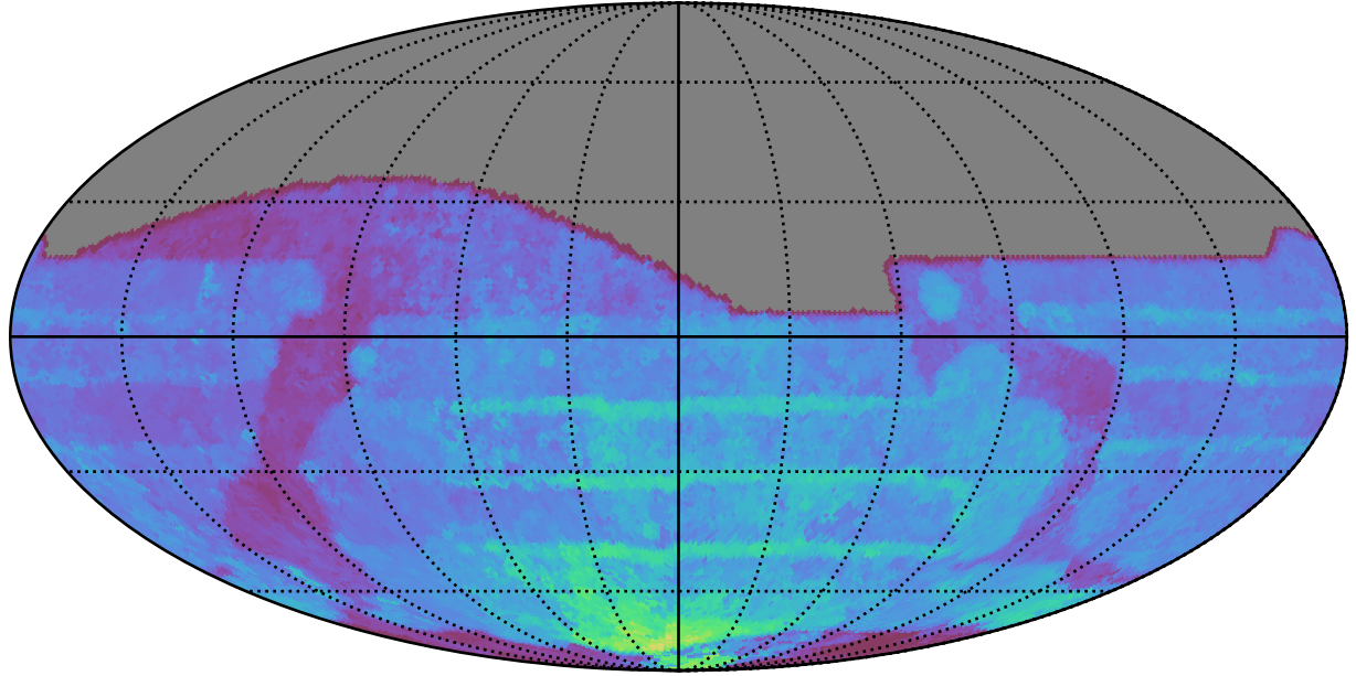
ddf_acor_sf15_lsf30_lsr10_v3.4_10yrs All sky all bands: 80thPercentile Season Length
