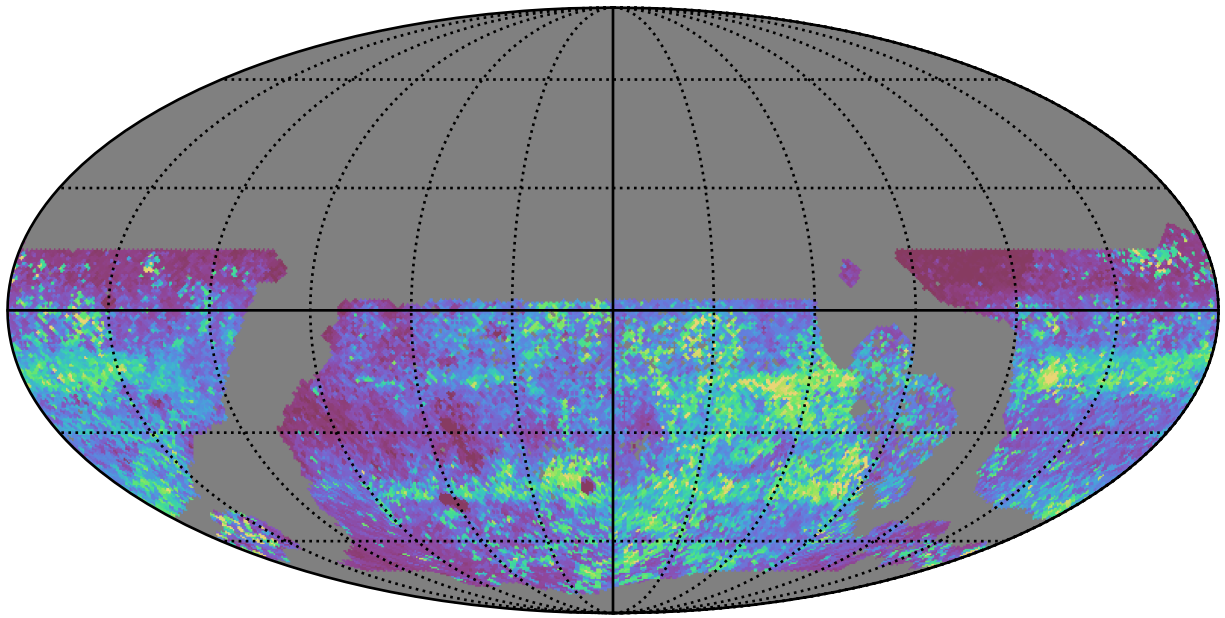
ddf_acor_sf15_lsf30_lsr10_v3.4_10yrs WFD zy bands: 75th Percentile Intranight Timespan
