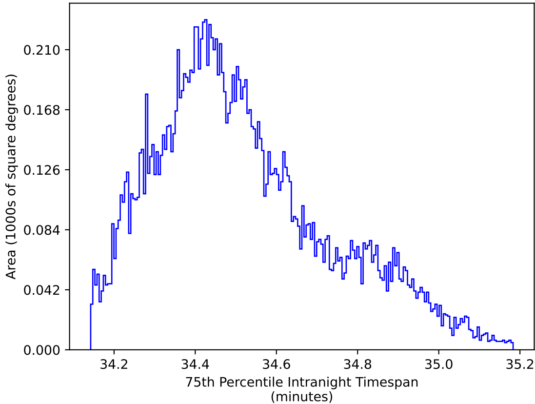
ddf_acor_sf15_lsf30_lsr10_v3.4_10yrs WFD zy bands: 75th Percentile Intranight Timespan
