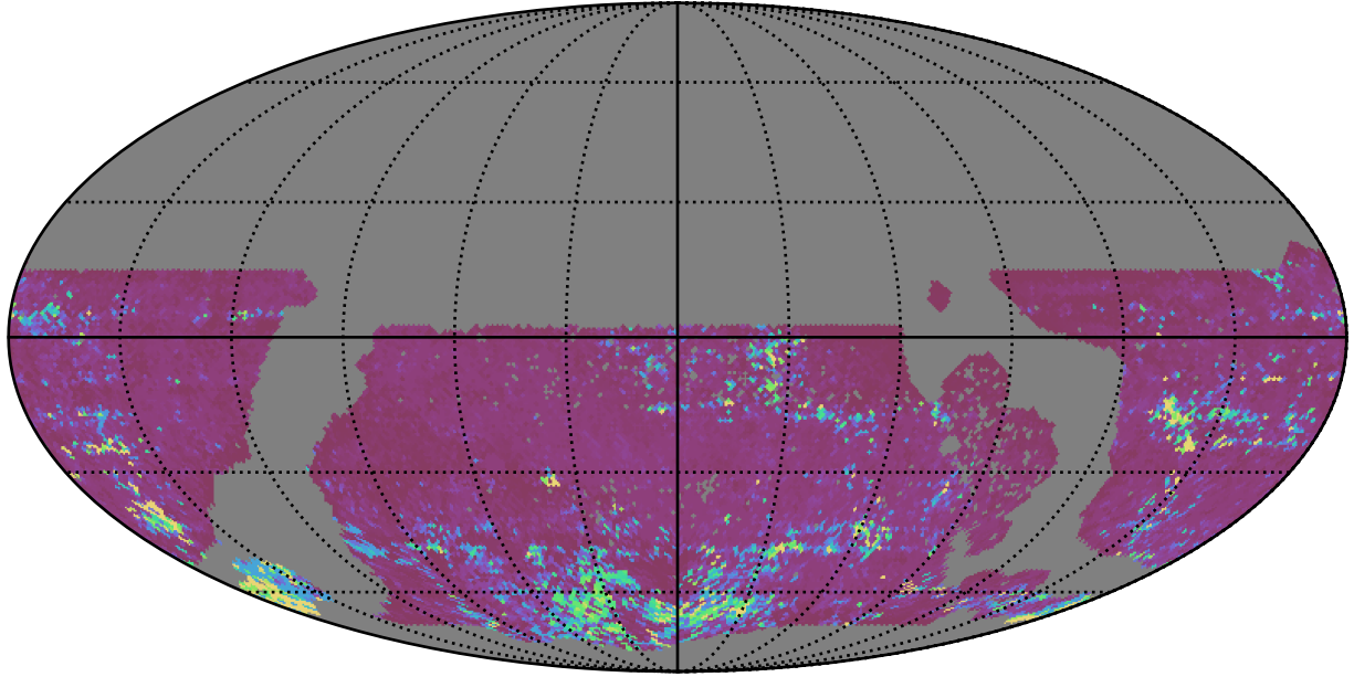
ddf_acor_sf15_lsf30_lsr10_v3.4_10yrs WFD z band: 75th Percentile Intranight Timespan
