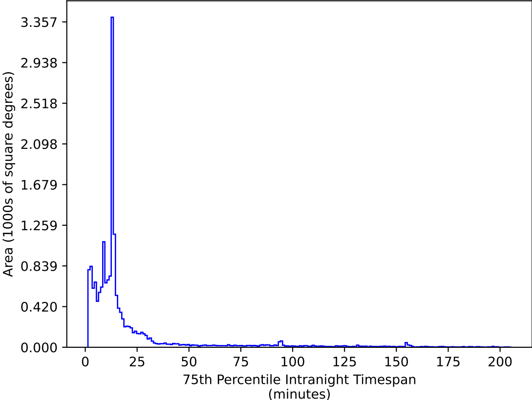
ddf_acor_sf15_lsf30_lsr10_v3.4_10yrs WFD z band: 75th Percentile Intranight Timespan
