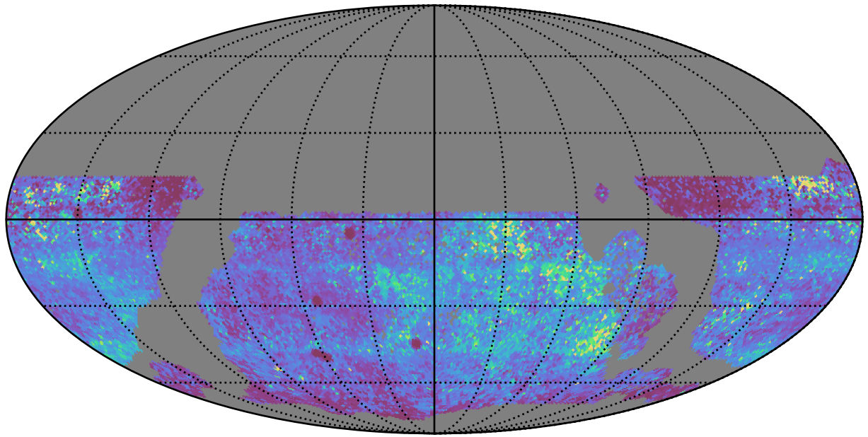
ddf_acor_sf15_lsf30_lsr10_v3.4_10yrs WFD y band: 75th Percentile Intranight Timespan
