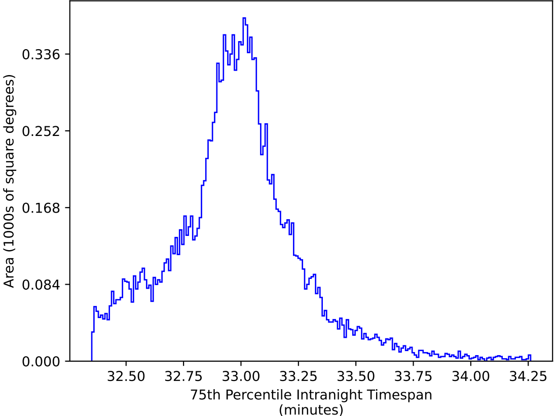
ddf_acor_sf15_lsf30_lsr10_v3.4_10yrs WFD y band: 75th Percentile Intranight Timespan
